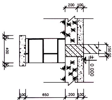
MÓNG MB ( TL 1.25)
